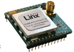
Figure 1: EVM-915-DTS Module
