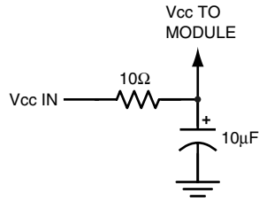
Figure 10: Supply Filter
